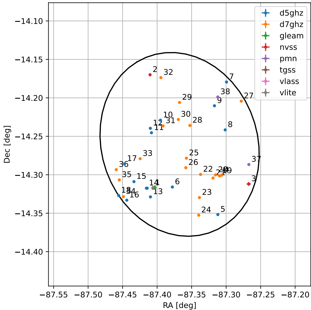
4FGL J1810.5-1415
