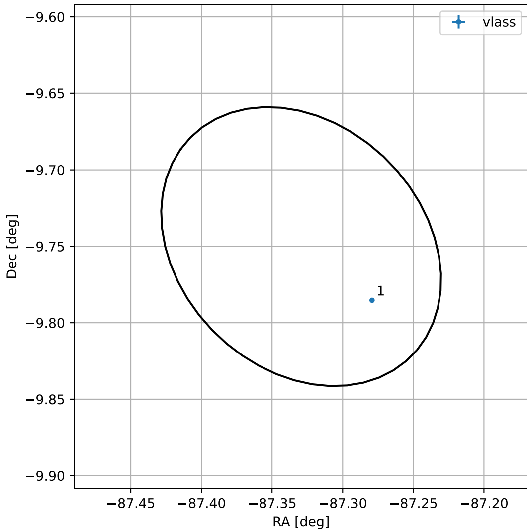
4FGL J1810.6-0945
