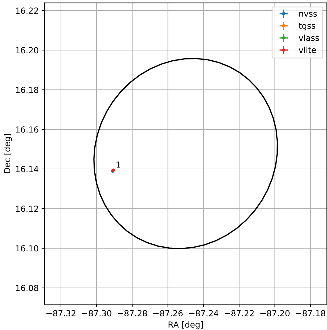
4FGL J1811.0+1608
