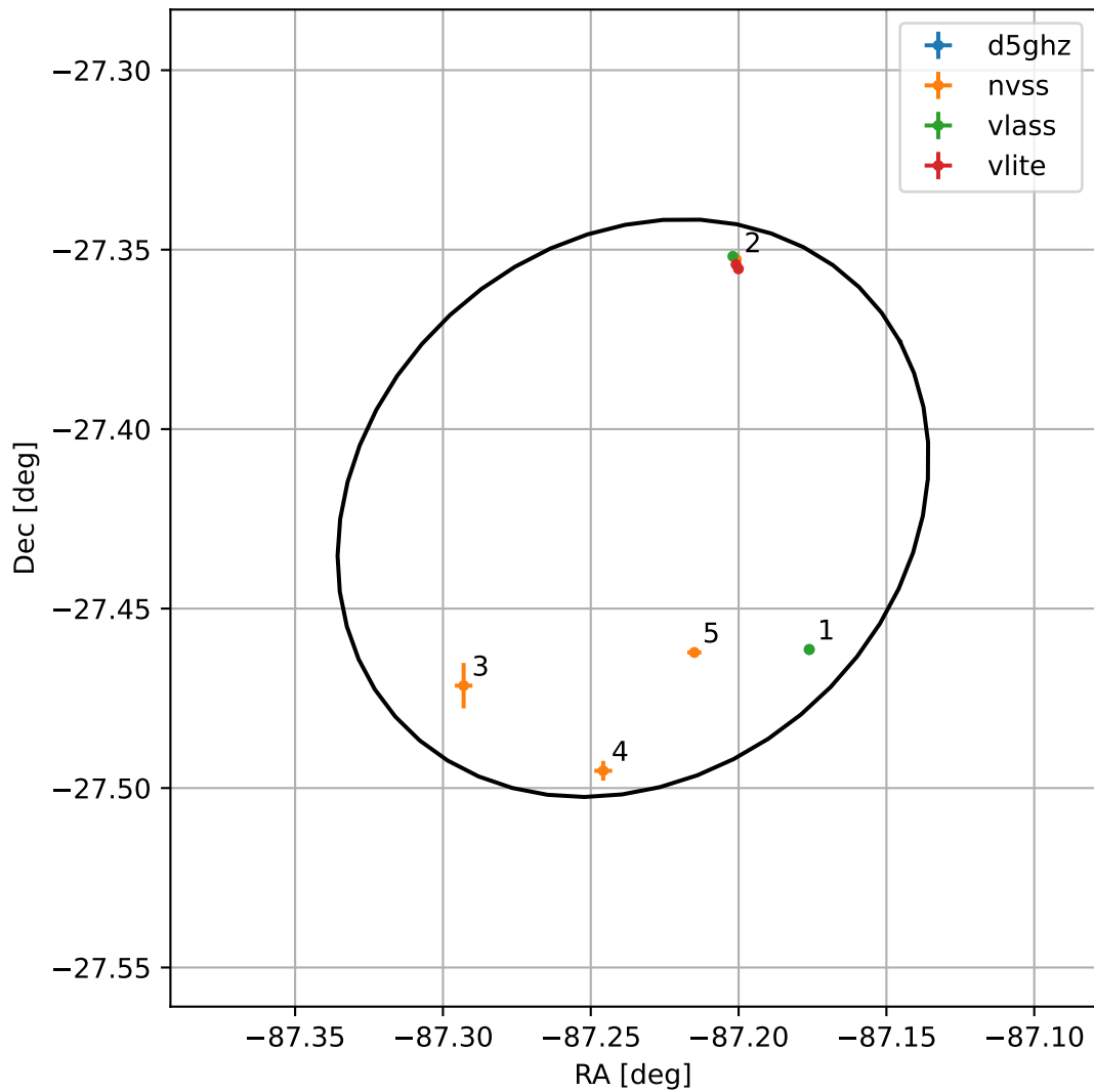
4FGL J1811.0-2725
