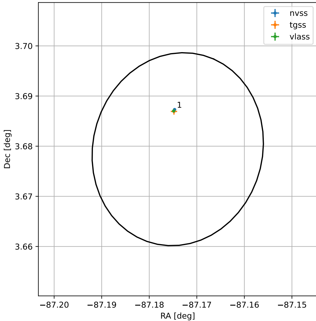
4FGL J1811.3+0340
