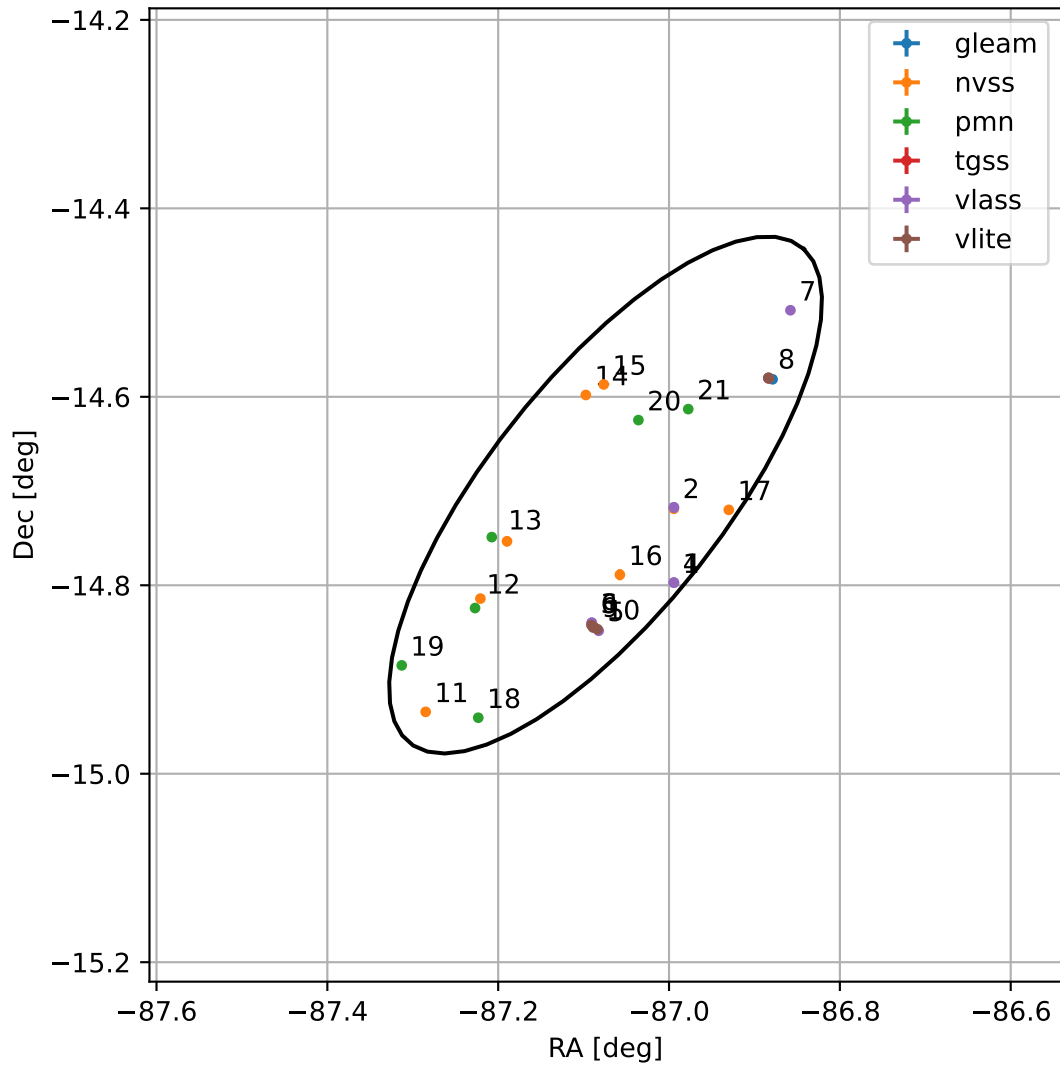
4FGL J1811.7-1442
