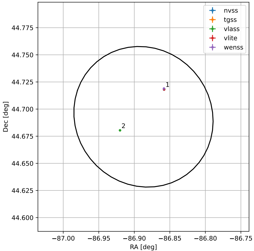
4FGL J1812.4+4441
