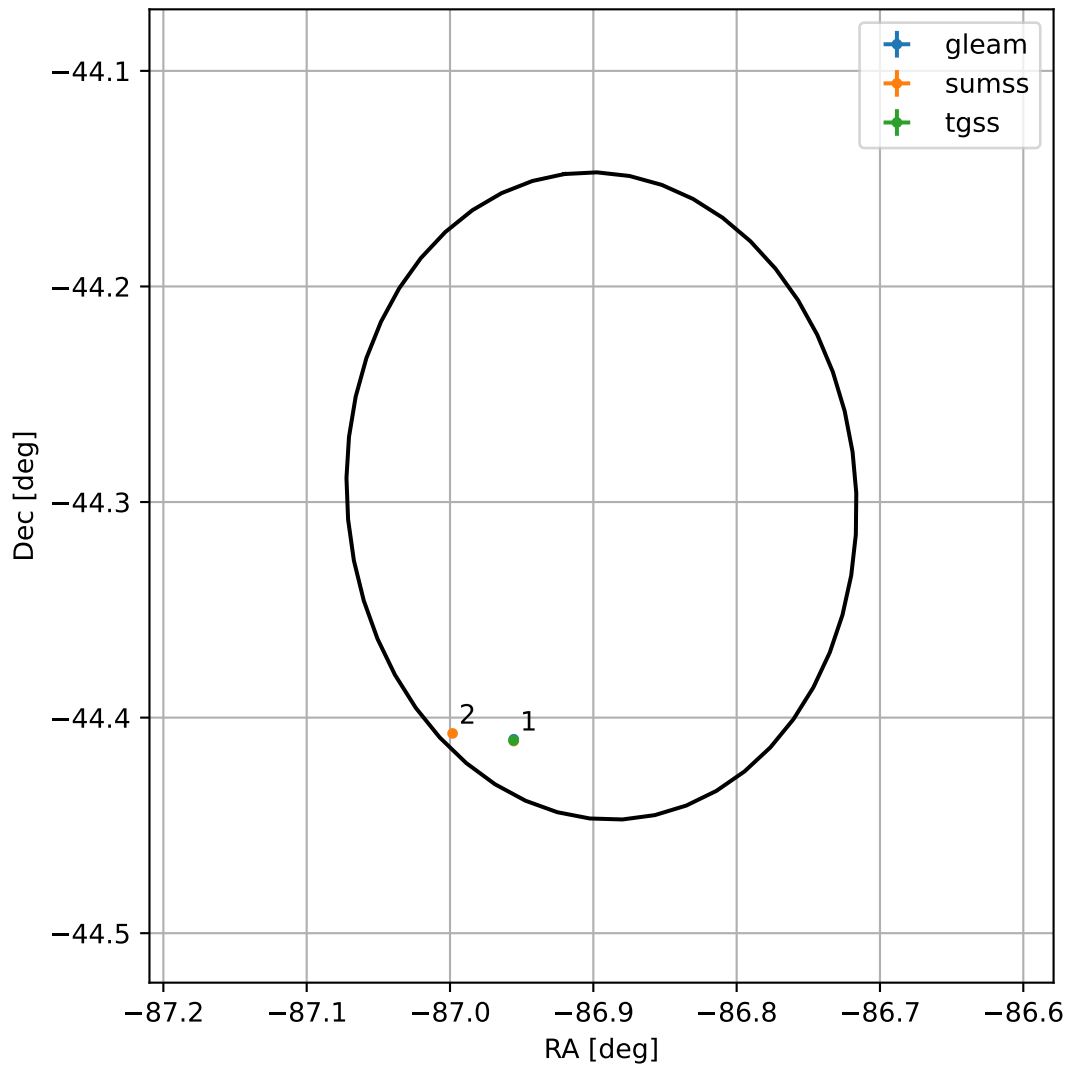
4FGL J1812.4-4417
