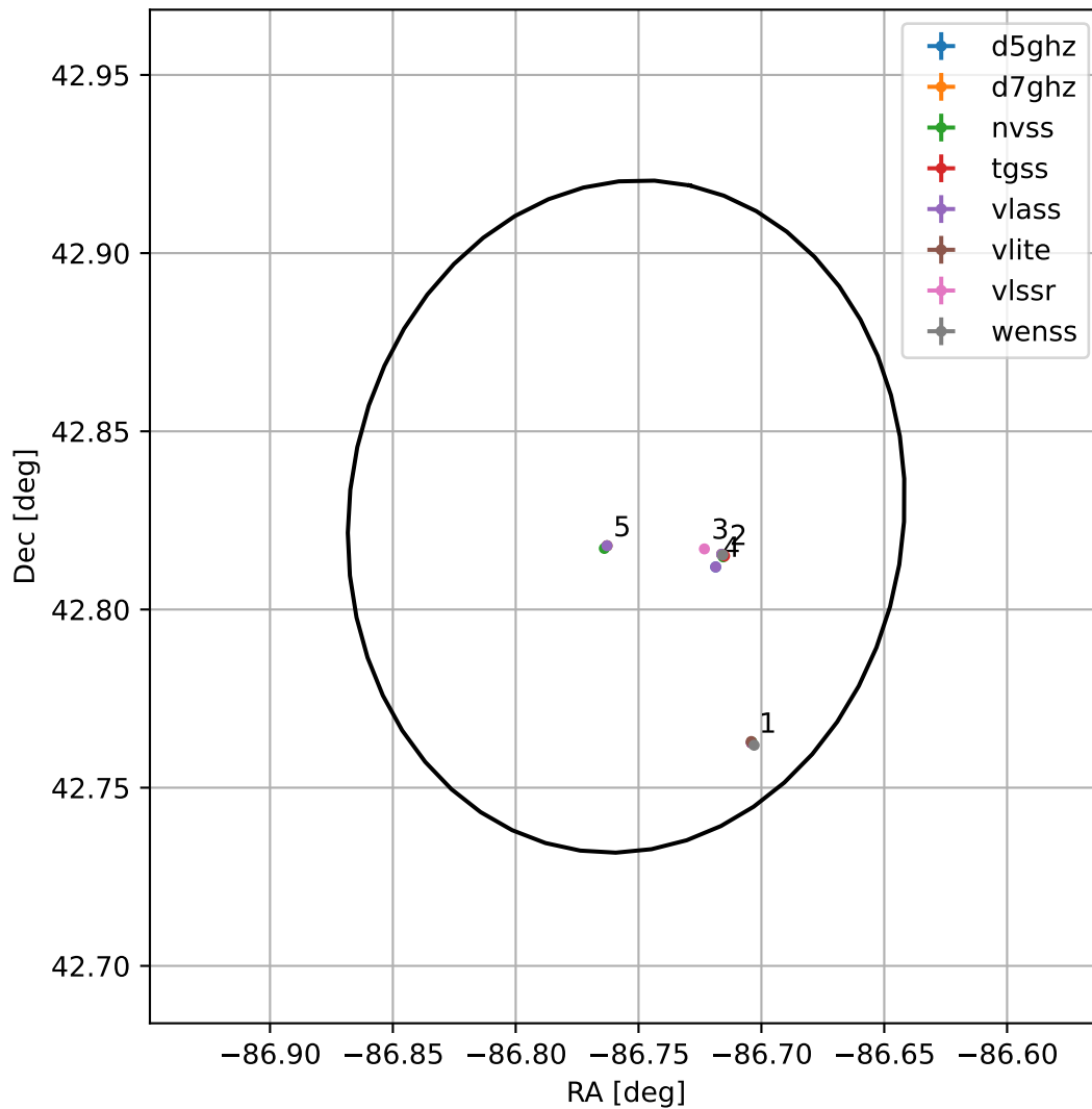
4FGL J1812.9+4249
