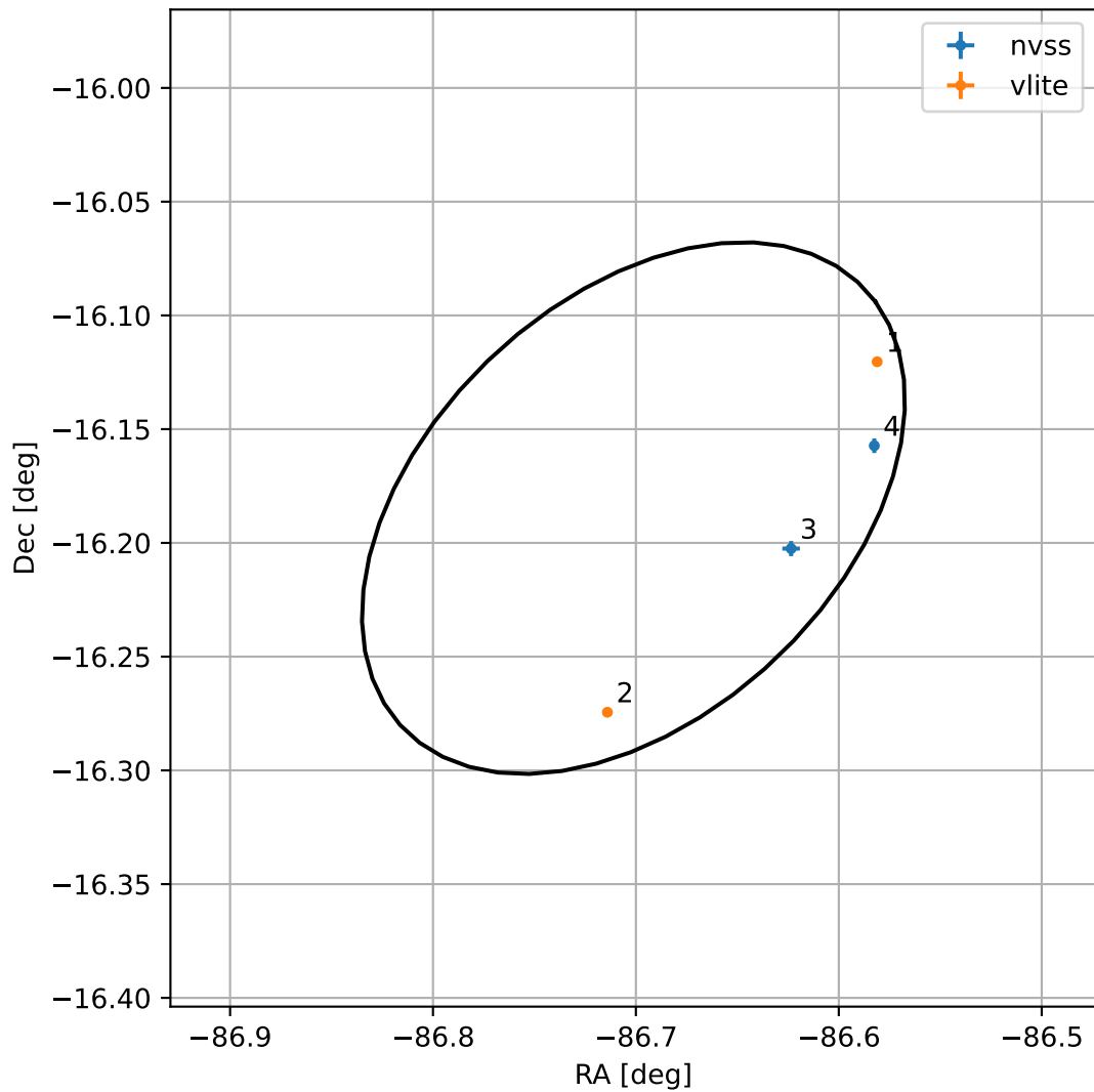
4FGL J1813.1-1611
