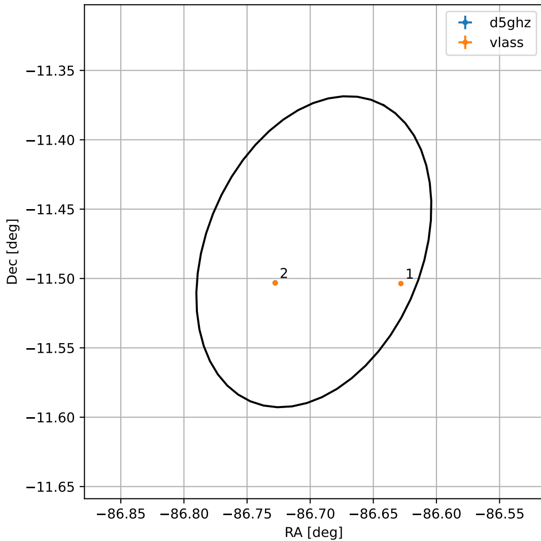
4FGL J1813.2-1128
