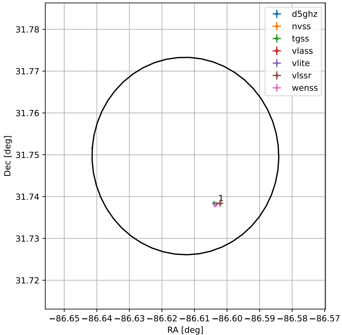
4FGL J1813.5+3144
