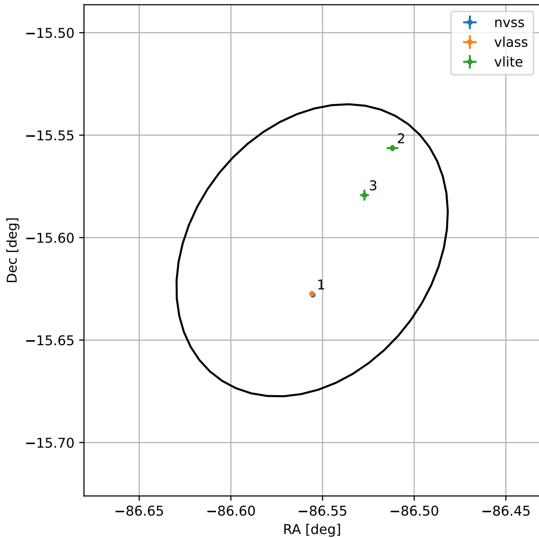
4FGL J1813.7-1536
