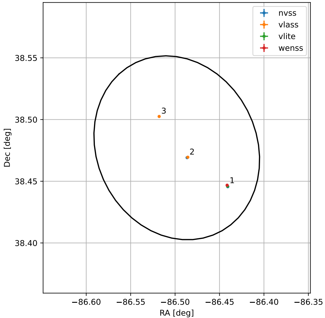
4FGL J1814.0+3828
