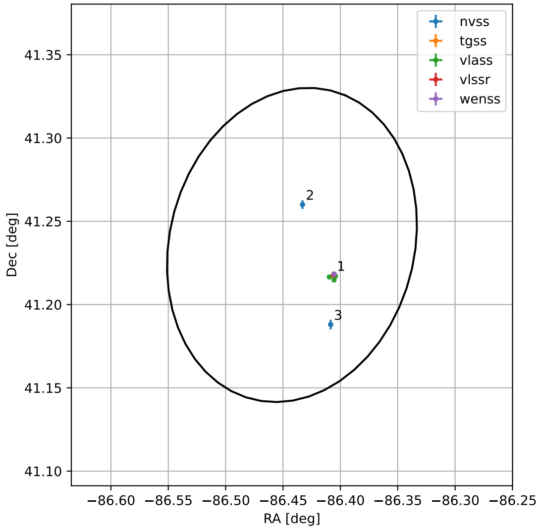
4FGL J1814.2+4114
