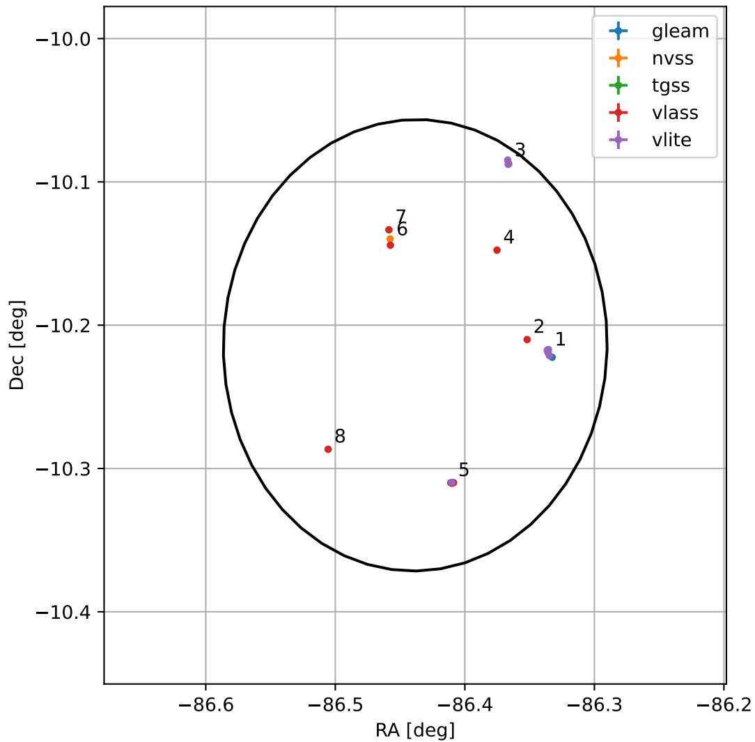
4FGL J1814.2-1012
