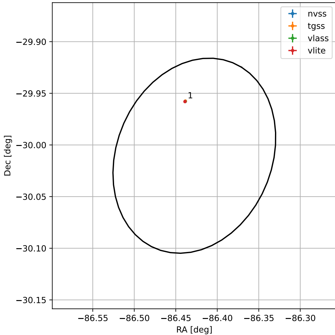
4FGL J1814.2-3000
