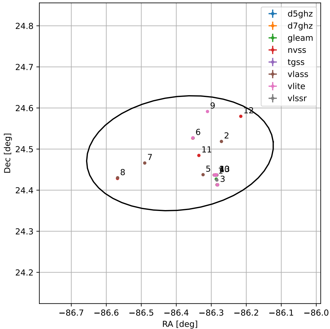
4FGL J1814.4+2429
