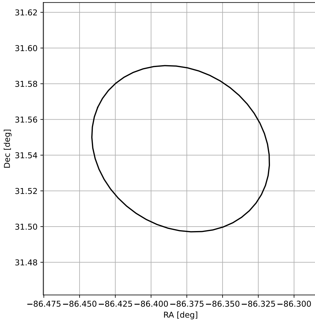
4FGL J1814.4+3132
