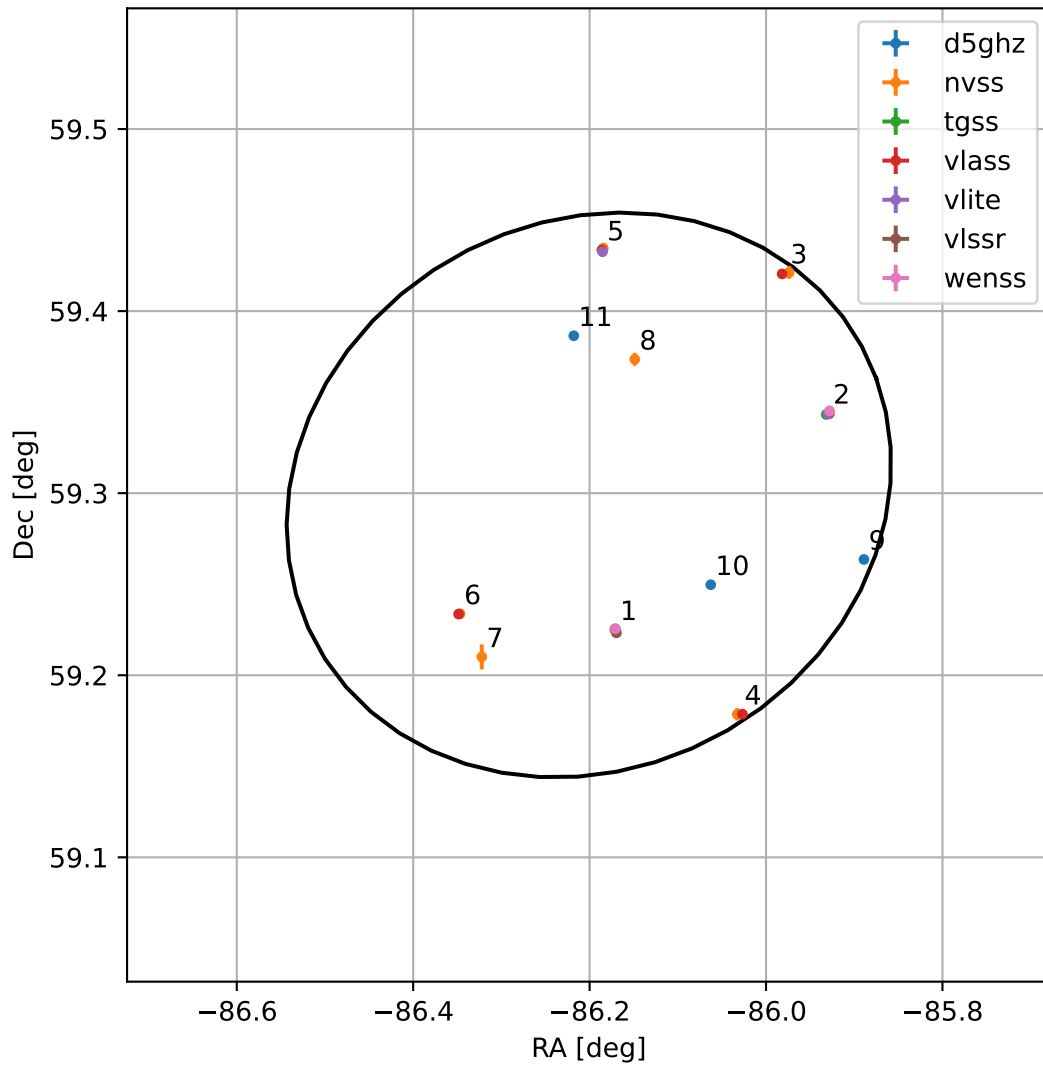
4FGL J1815.1+5917
