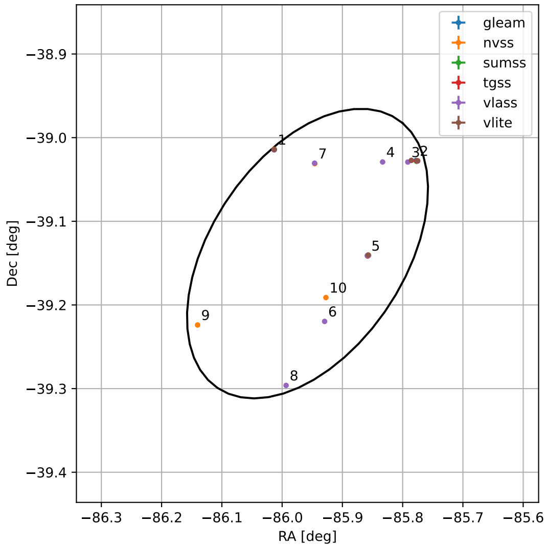
4FGL J1816.1-3908
