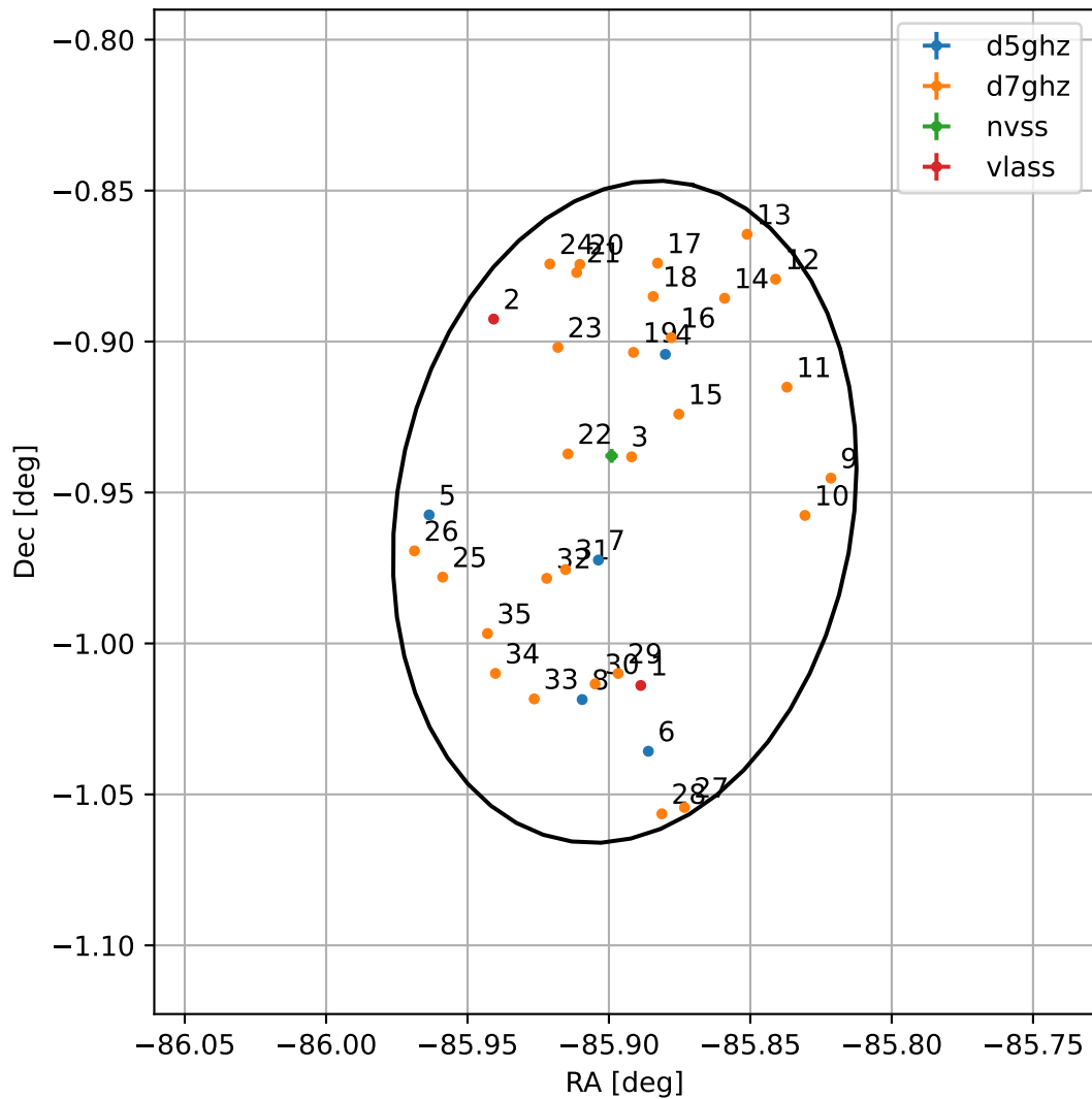
4FGL J1816.4-0057
