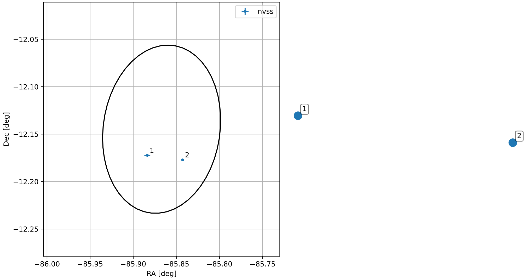
4FGL J1816.5-1208
