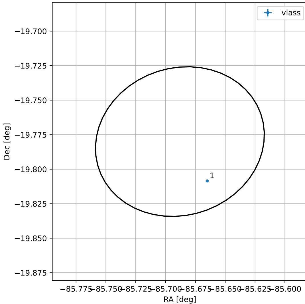
4FGL J1817.2-1946
