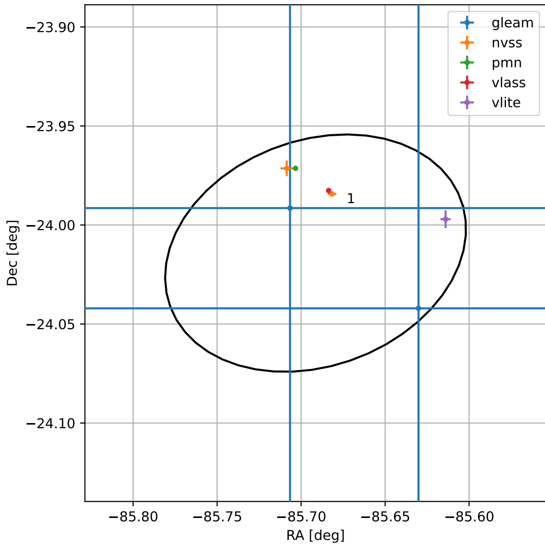
4FGL J1817.2-2400
