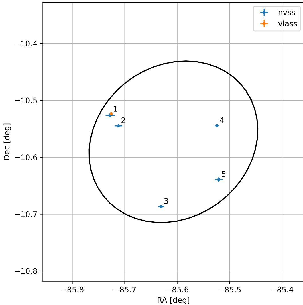
4FGL J1817.5-1034
