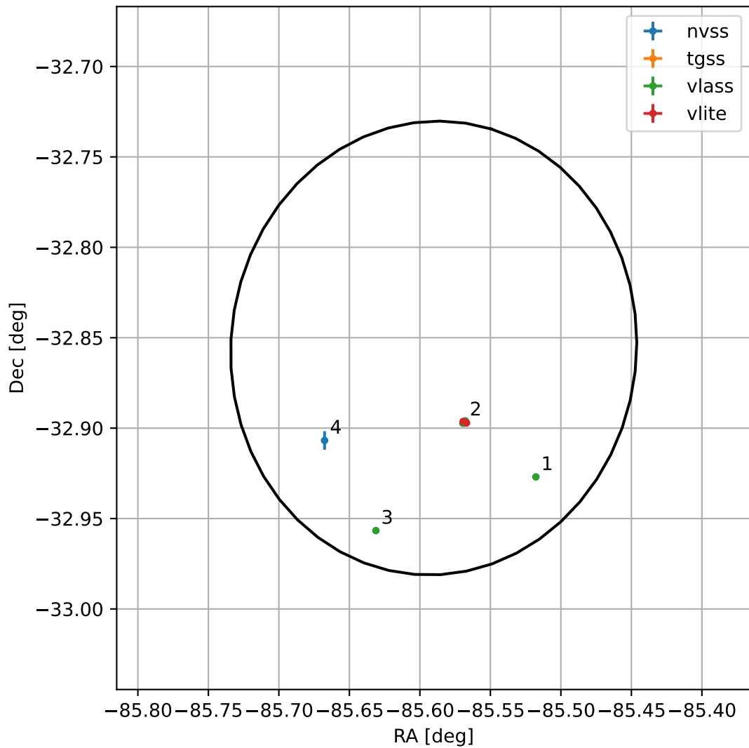
4FGL J1817.6-3251
