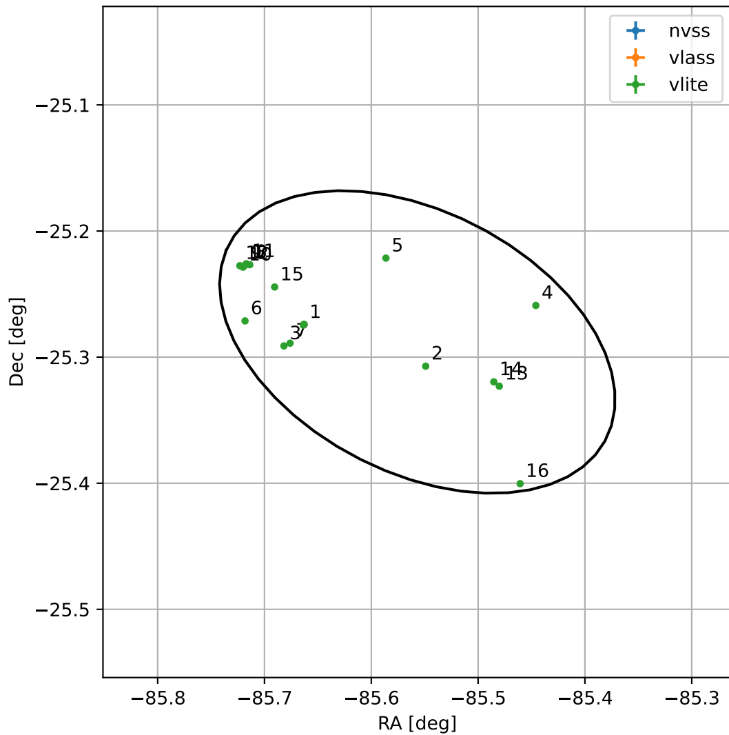
4FGL J1817.7-2517
