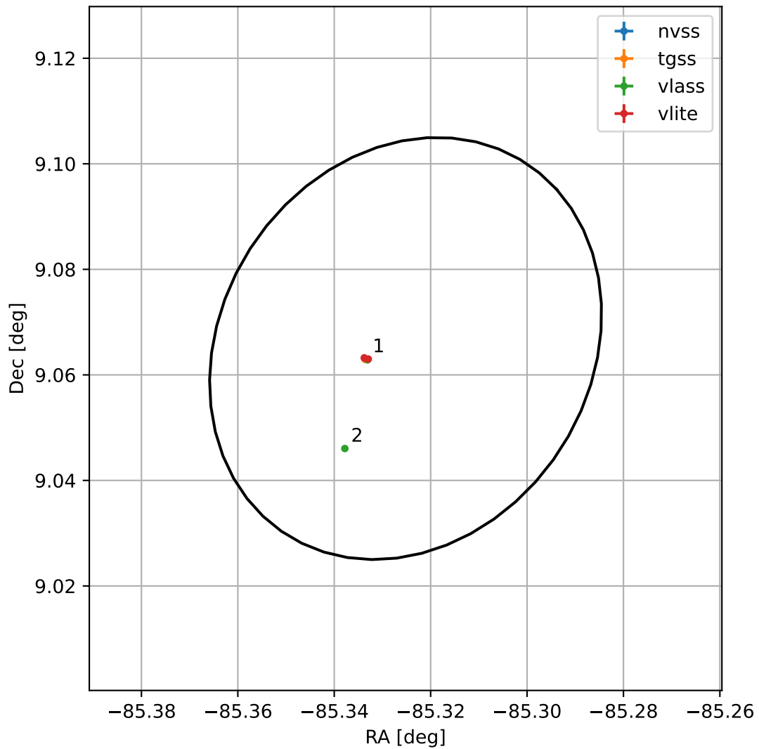
4FGL J1818.6+0903
