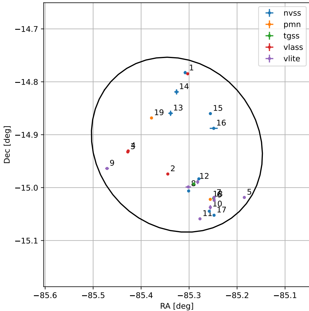
4FGL J1818.6-1455
