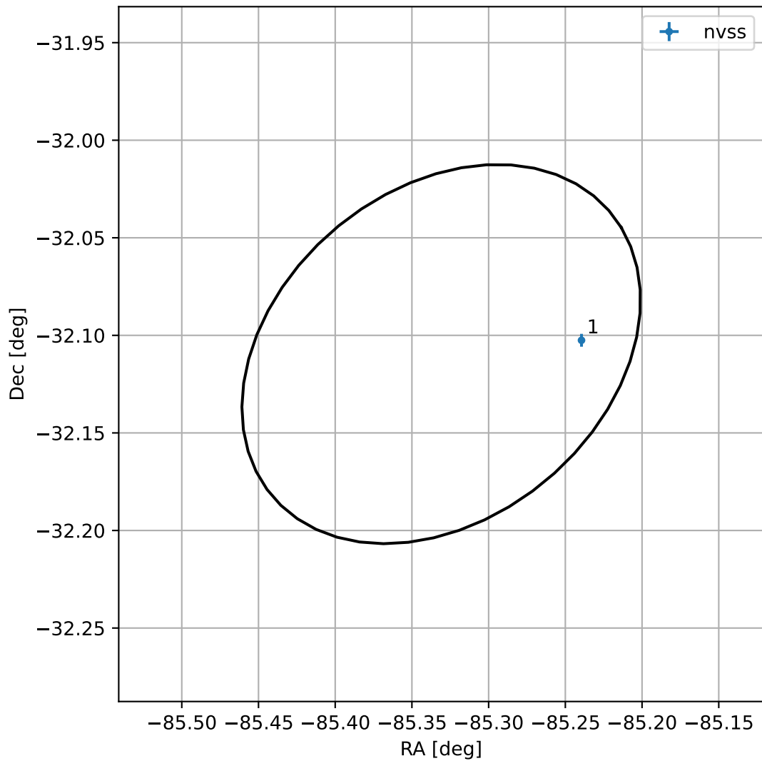
4FGL J1818.6-3206
