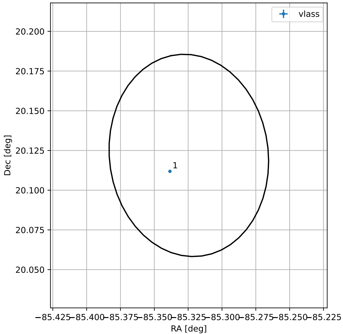
4FGL J1818.7+2007
