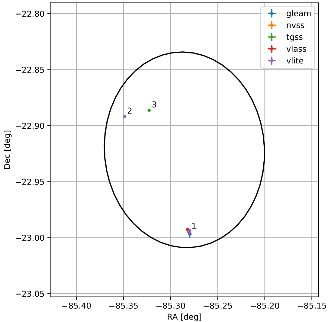
4FGL J1818.8-2255
