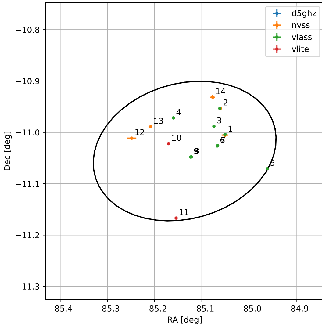
4FGL J1819.4-1102
