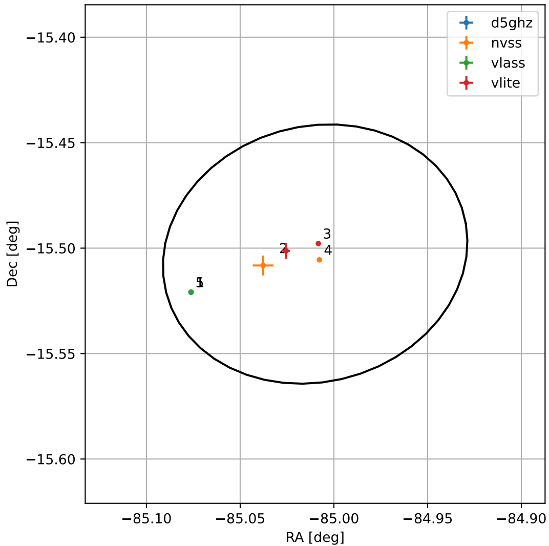
4FGL J1819.9-1530
