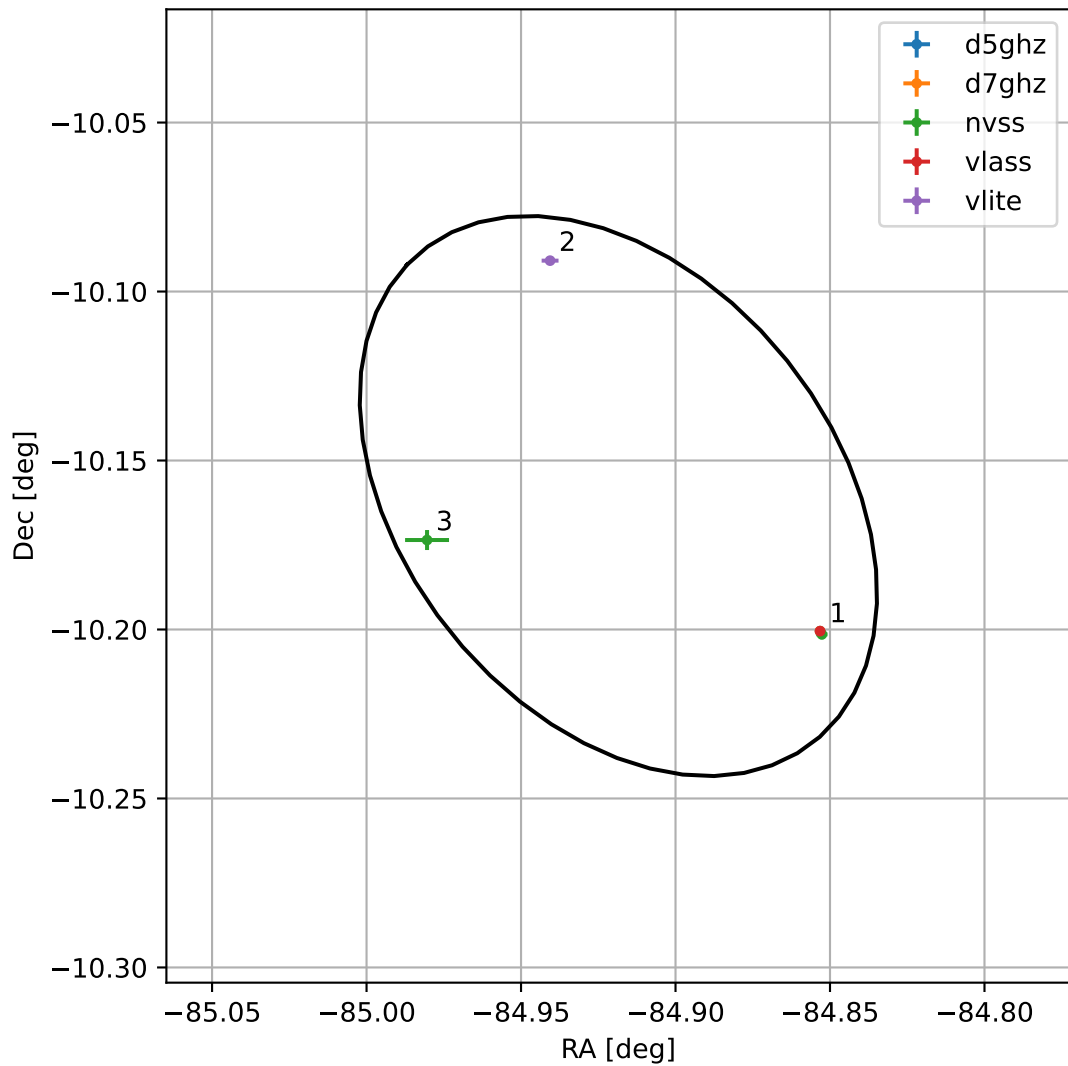
4FGL J1820.3-1009
