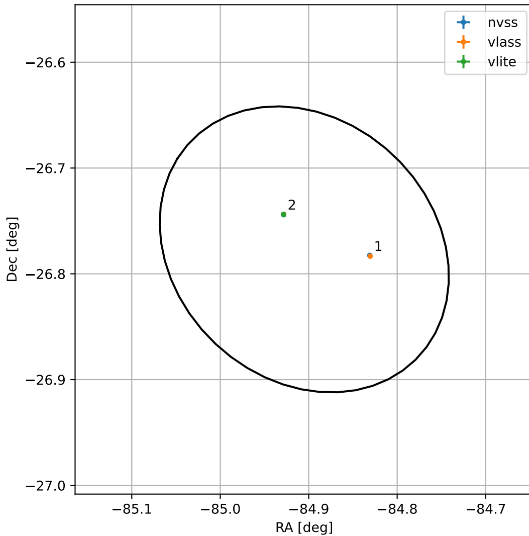
4FGL J1820.3-2646
