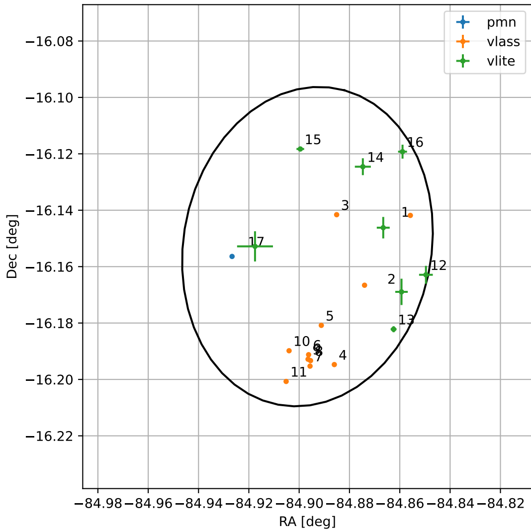
4FGL J1820.4-1609
