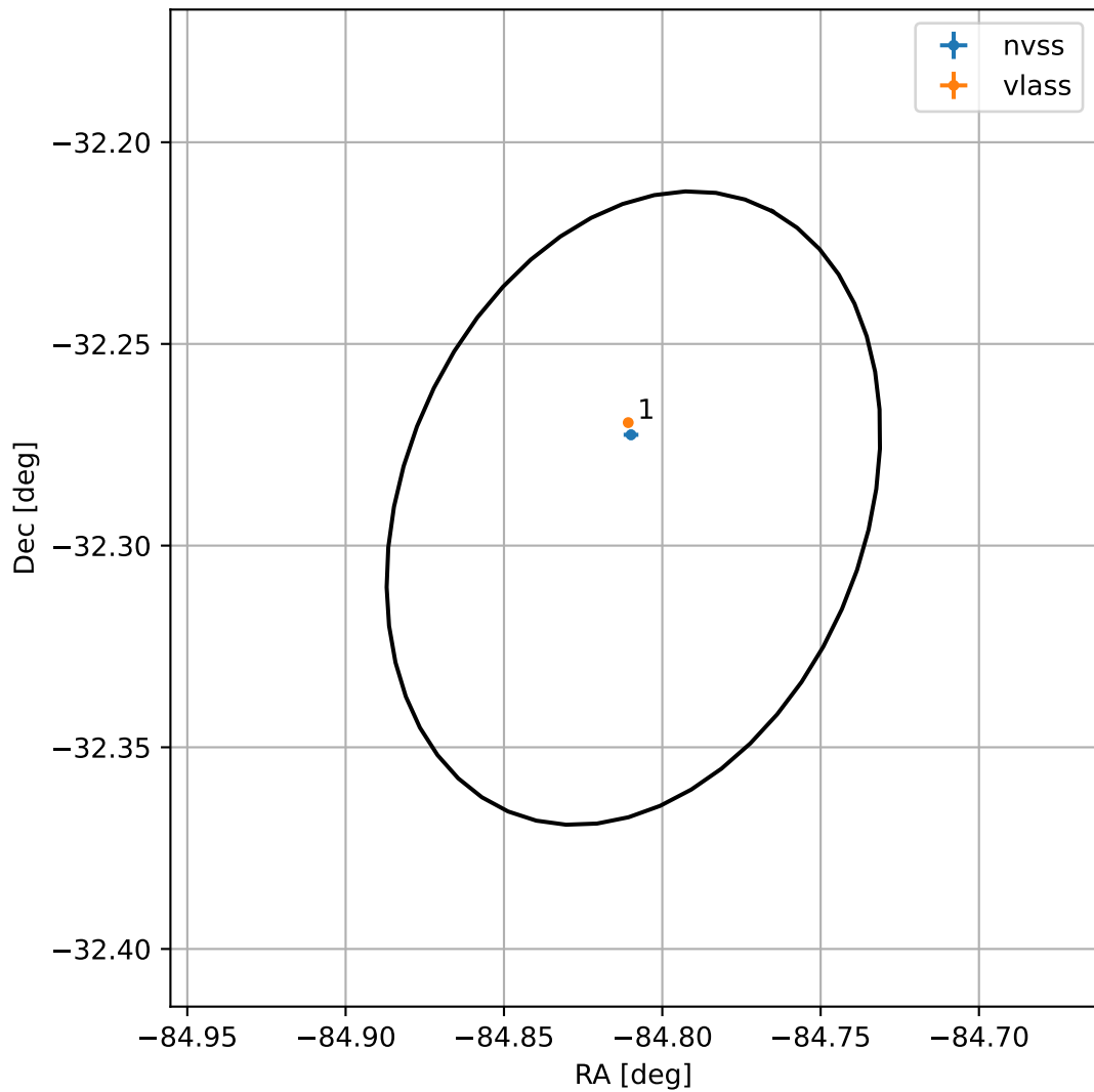
4FGL J1820.7-3217
