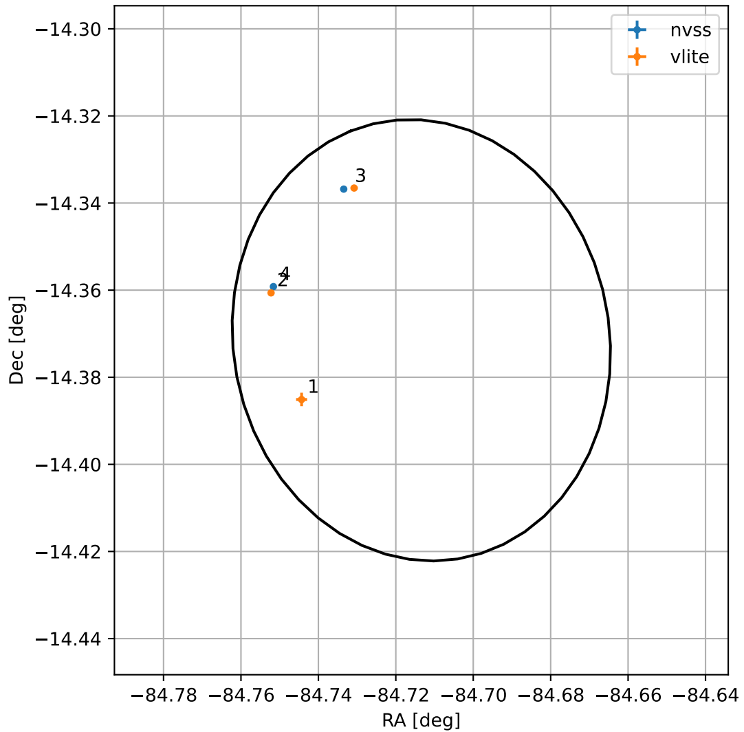
4FGL J1821.1-1422
