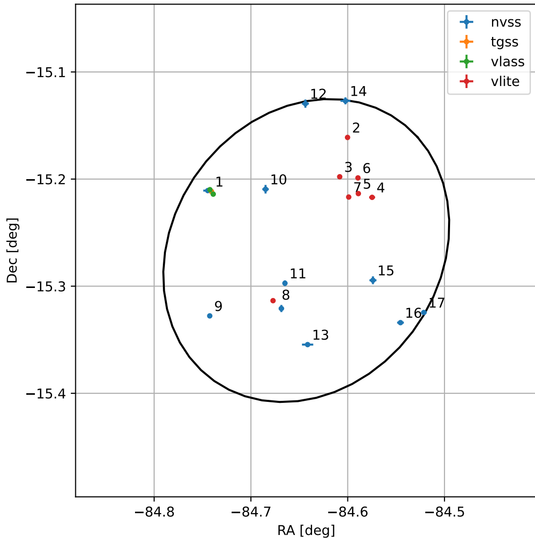
4FGL J1821.4-1516
