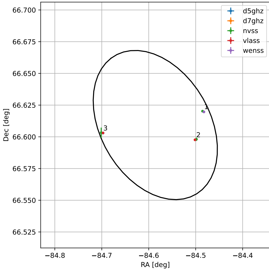
4FGL J1821.6+6636
