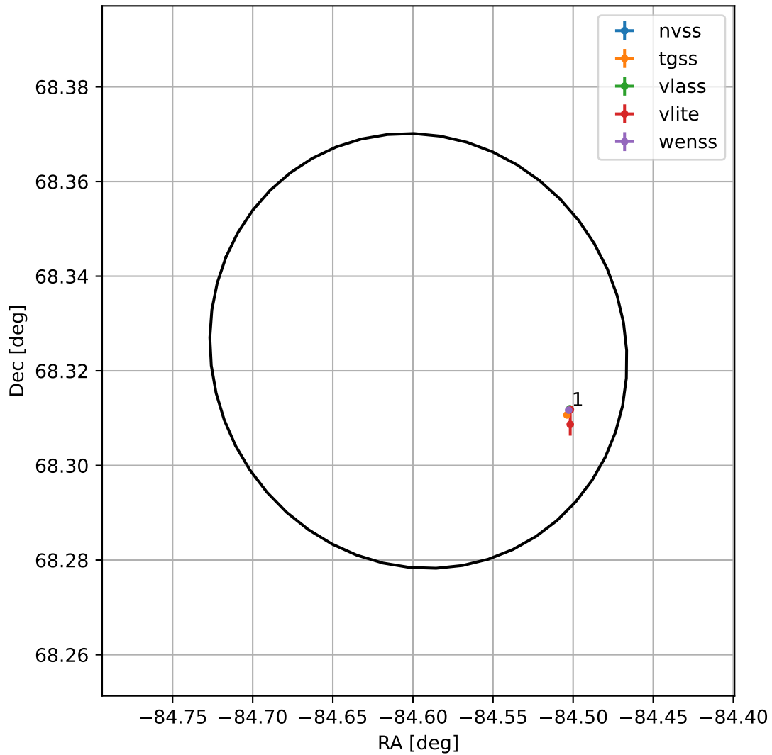
4FGL J1821.6+6819
