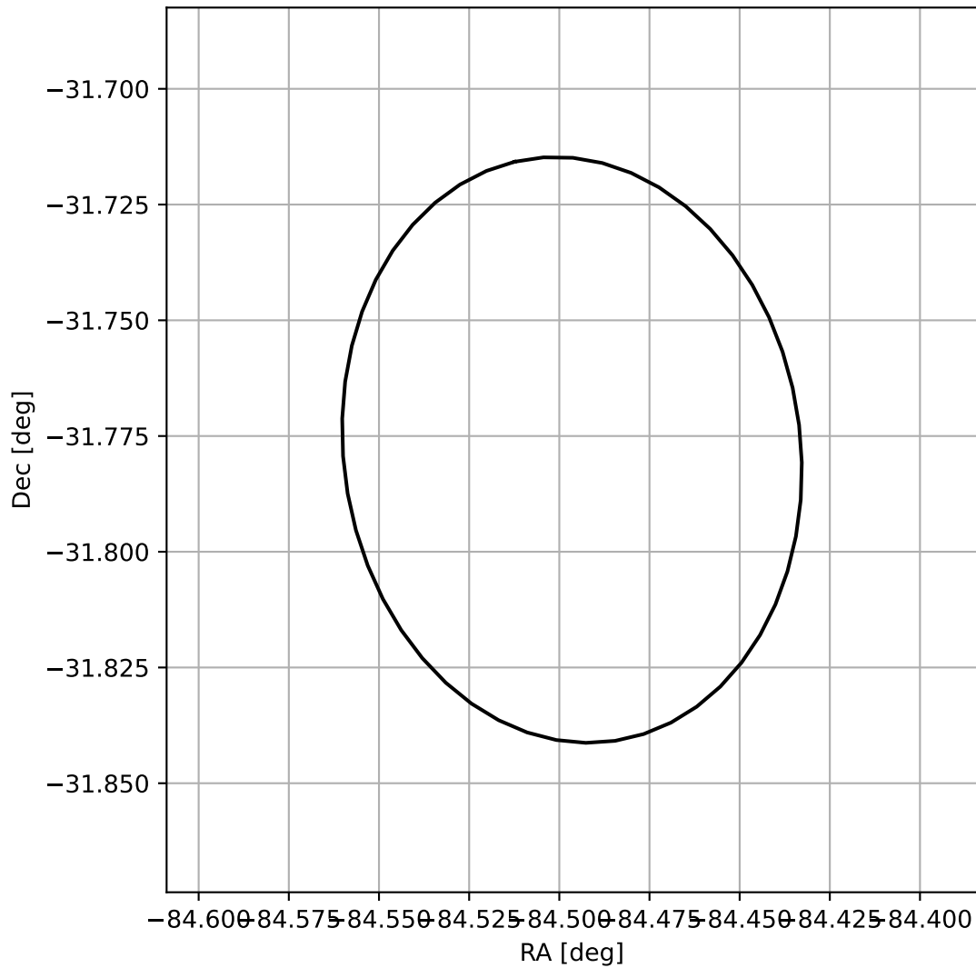
4FGL J1822.0-3146
