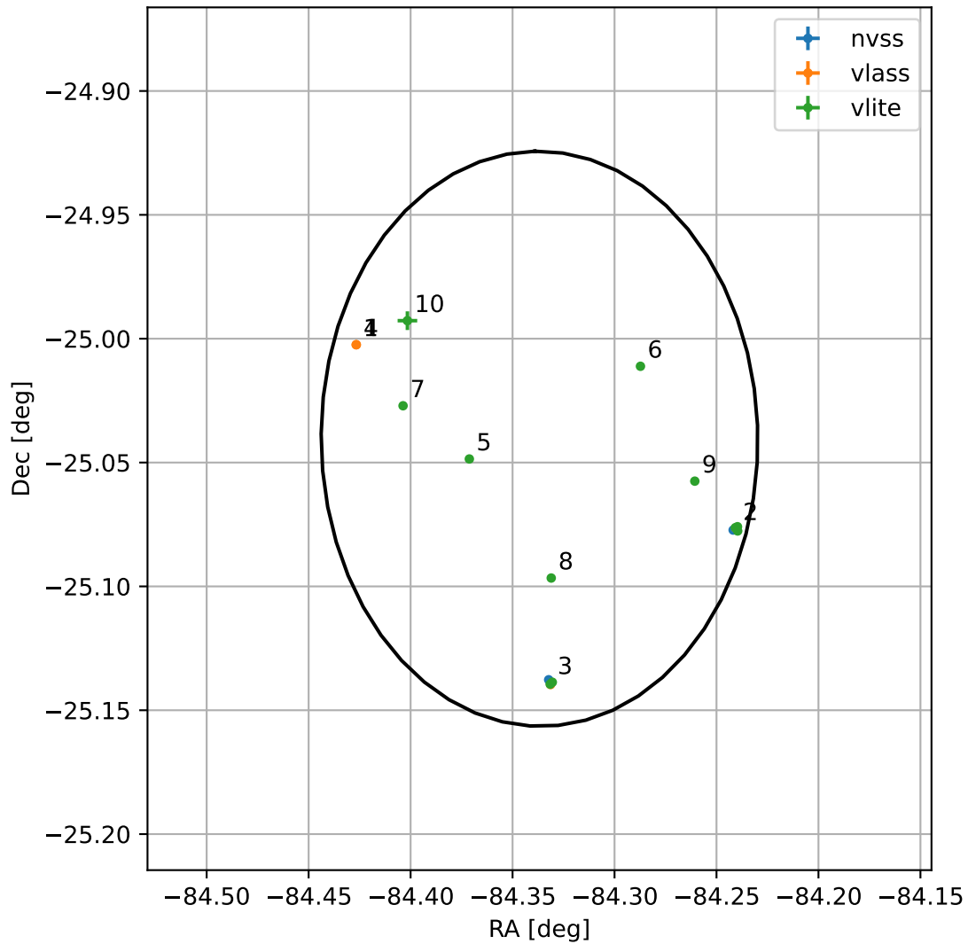
4FGL J1822.6-2502
