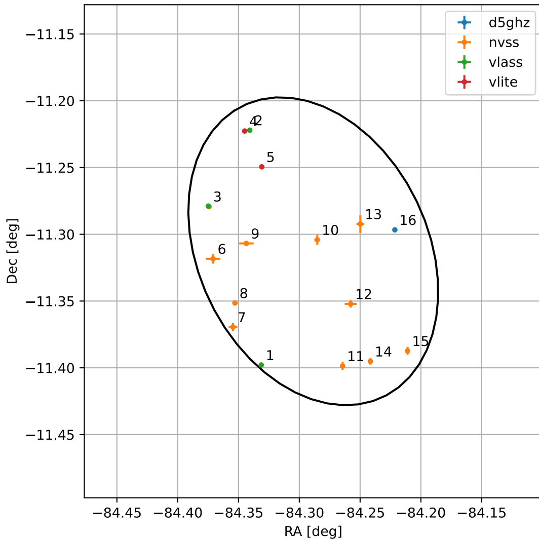
4FGL J1822.8-1118
