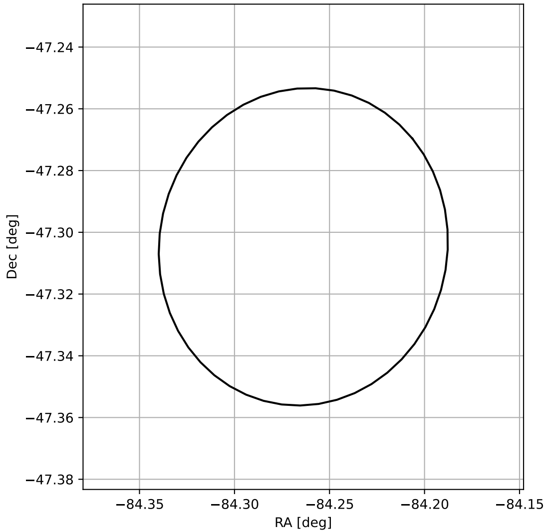
4FGL J1822.9-4718
