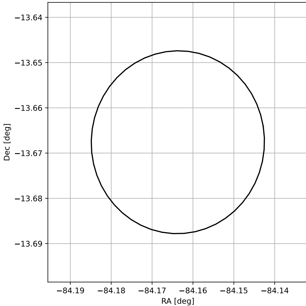
4FGL J1823.3-1340
