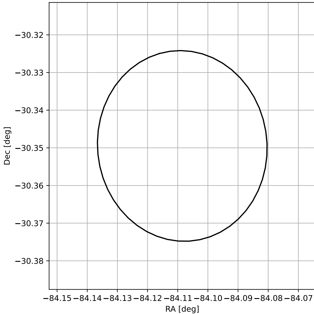
4FGL J1823.5-3020
