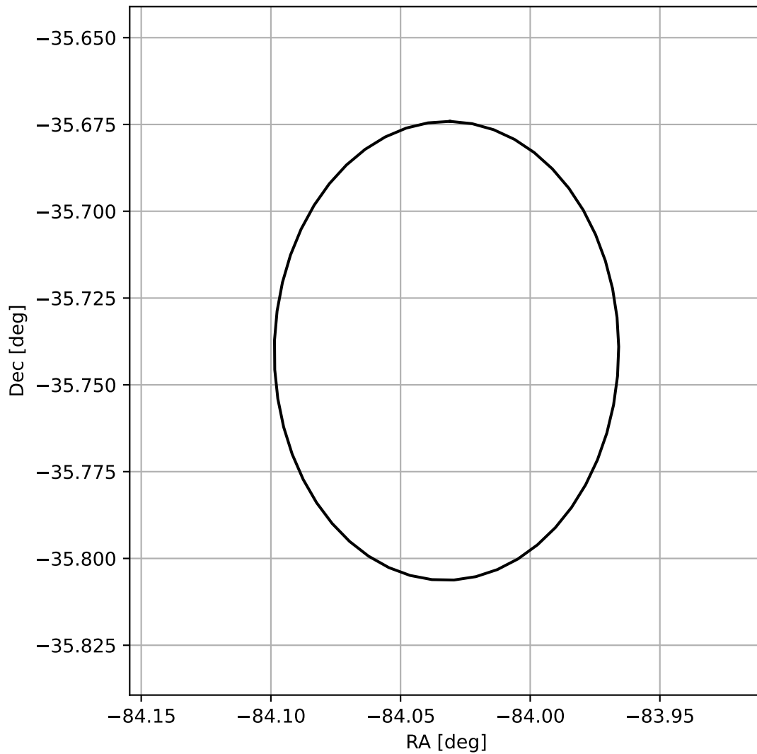
4FGL J1823.8-3544
